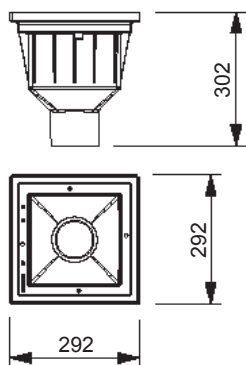
MEAPARK Bodová vpust'
